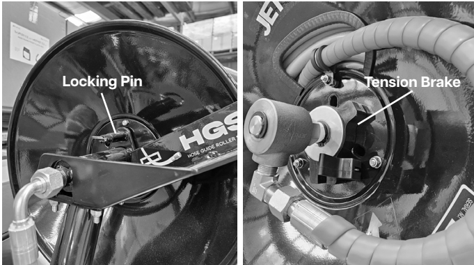
Figure.9 - Brake Adjustment
